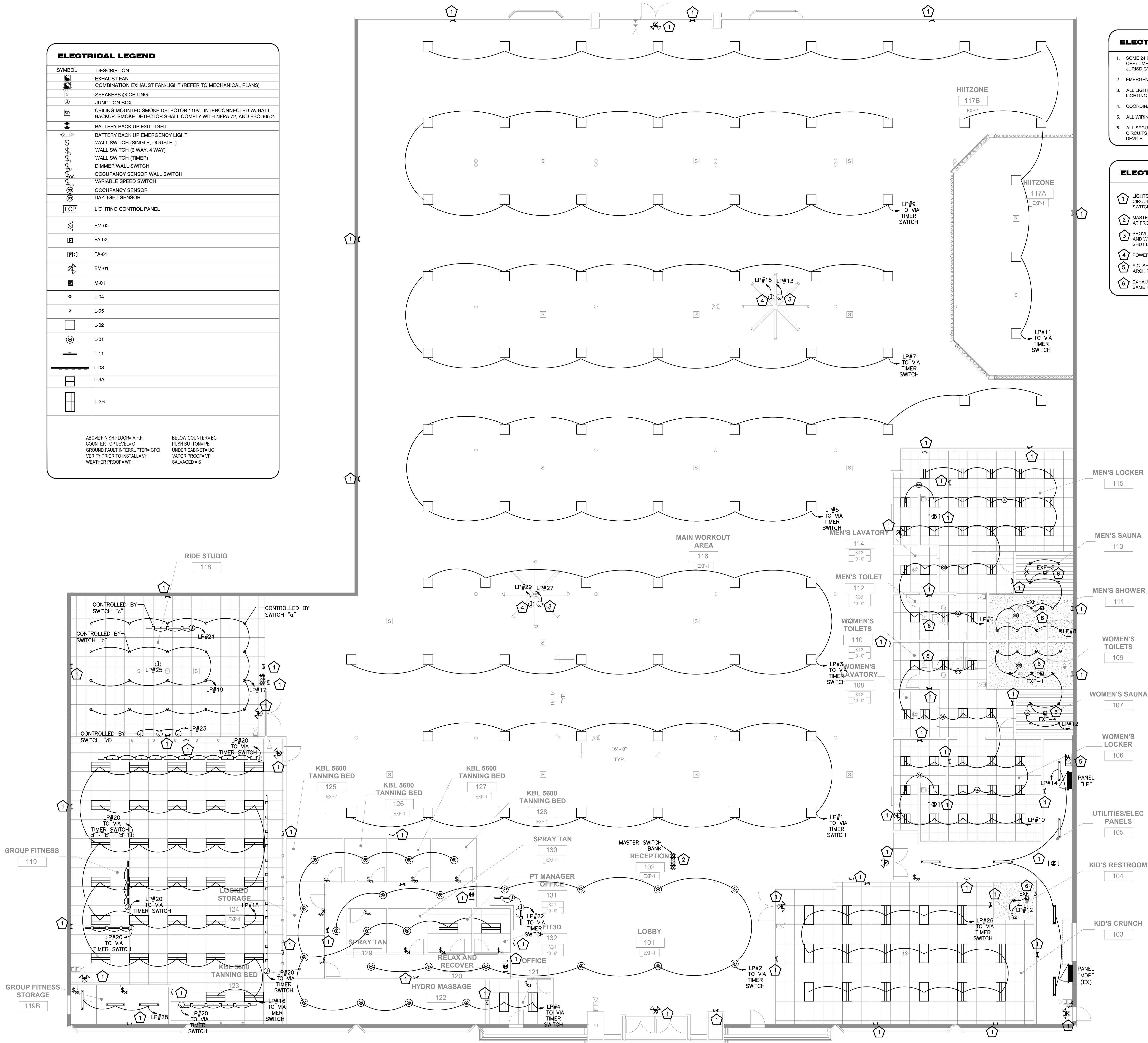
1 ELECTRICAL LIGHTING FLOOR PLAN 1/8" = 1'-0"
