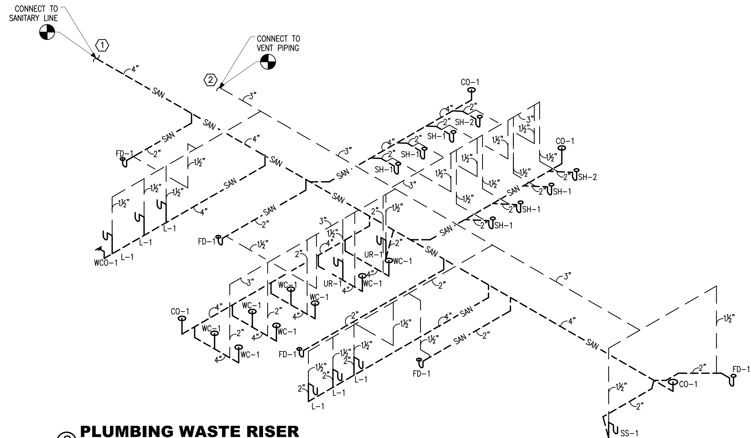
② PLUMBING WASTE RISER NTS
