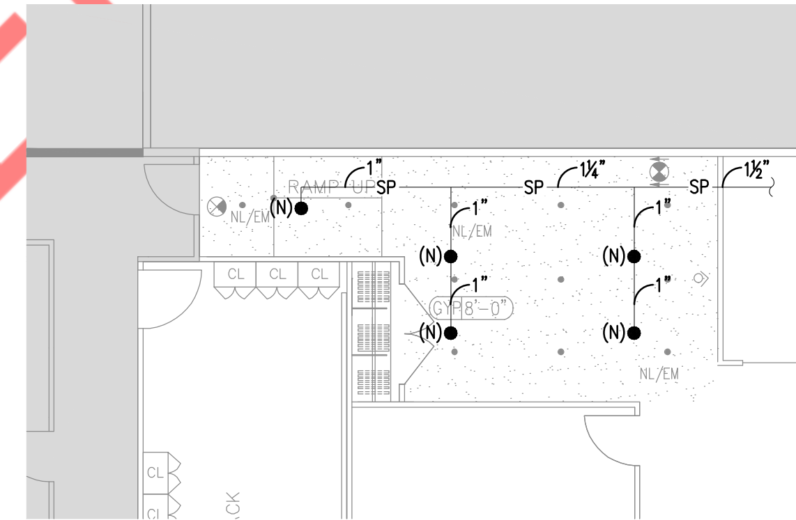
1 SPRINKLER ALTERNATE RECEPTION AREA SCALE: 1/8" = 1'-0"
