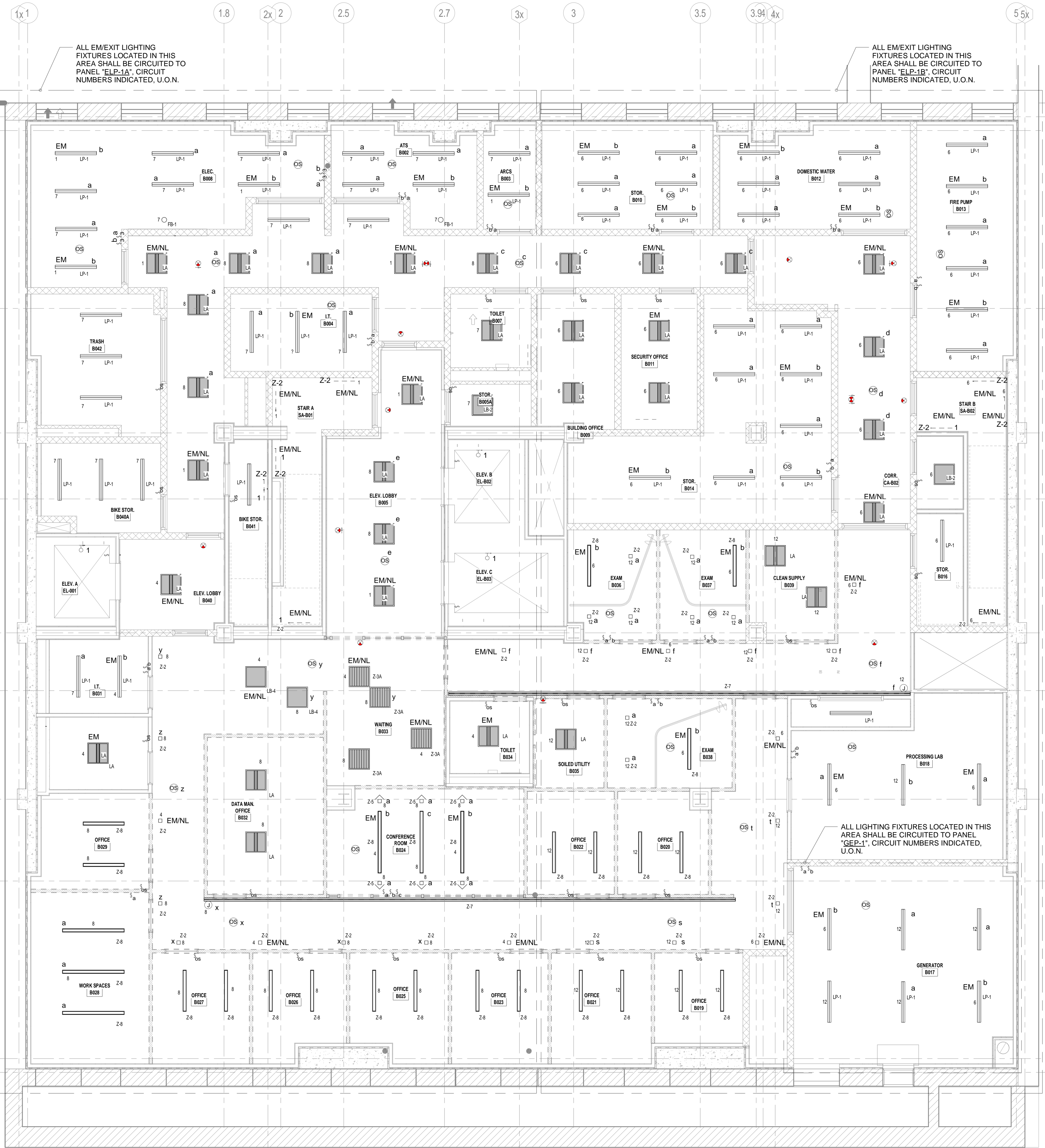
1) CELLAR LIGHTING PLAN 1/4" = 1'-0"
