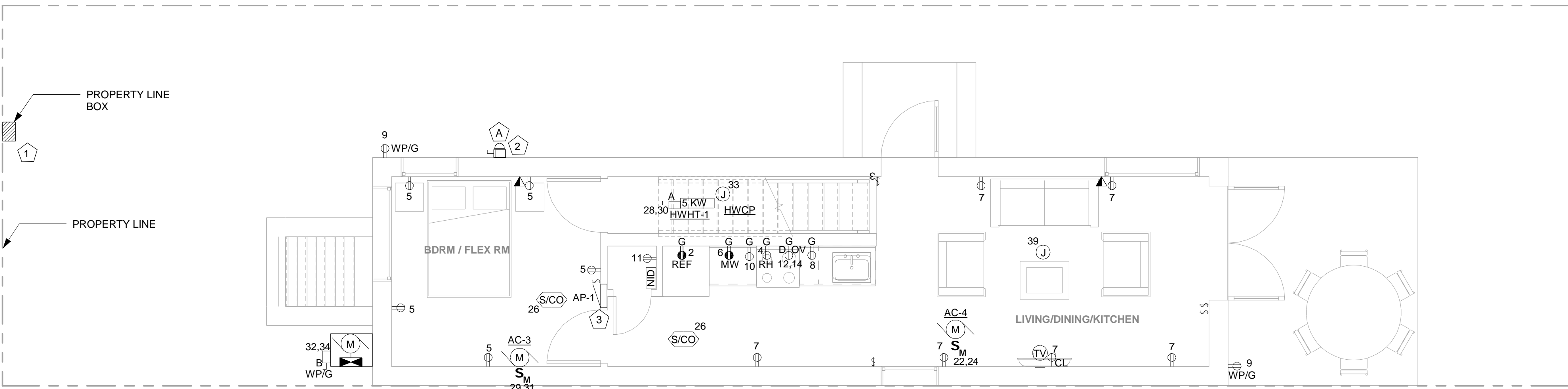
1 1ST FLOOR ELECTRICAL POWER PLAN 1/4" = 1'-0"
