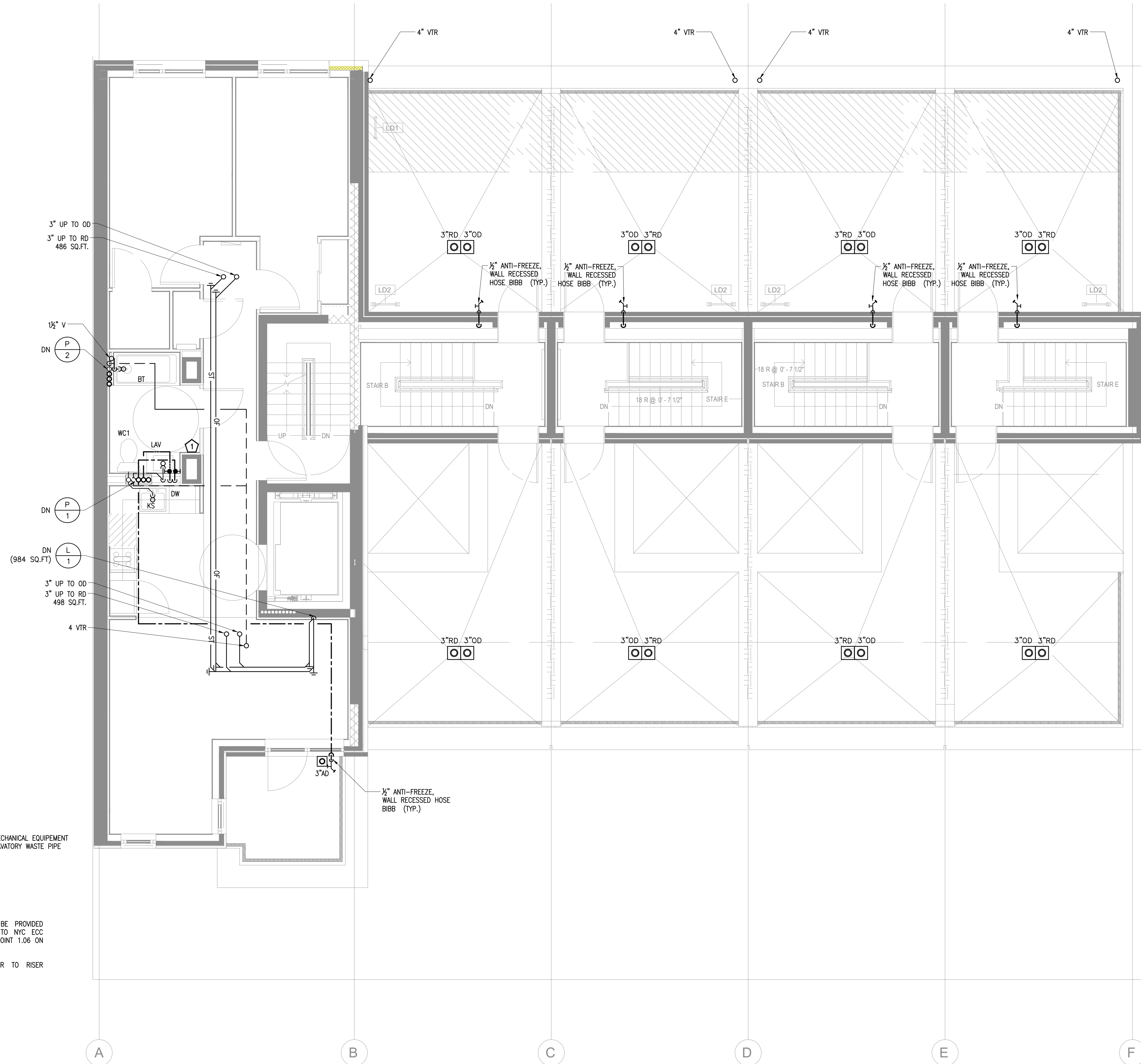
1 5TH FLOOR PLUMBING PLAN 1/4" = 1'-0"
