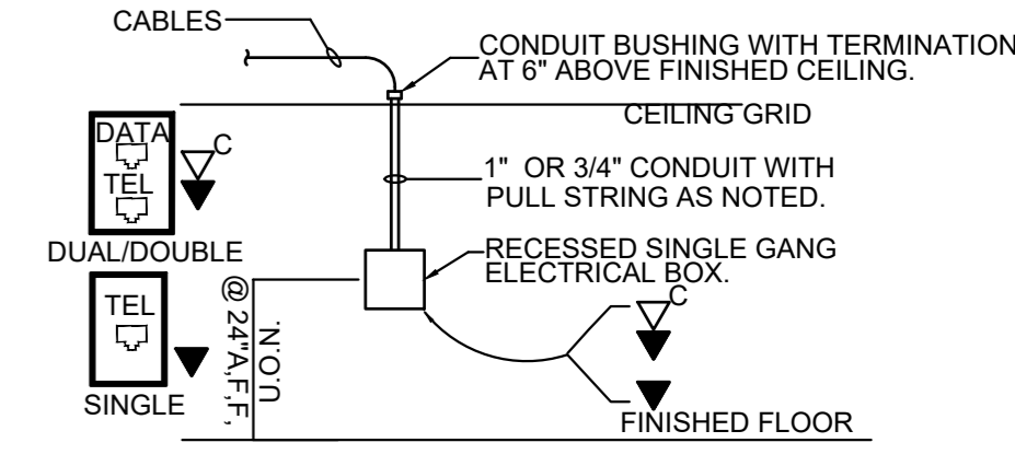
3 TYP COMM. STUB UP DETAIL E-201.00 NTS
