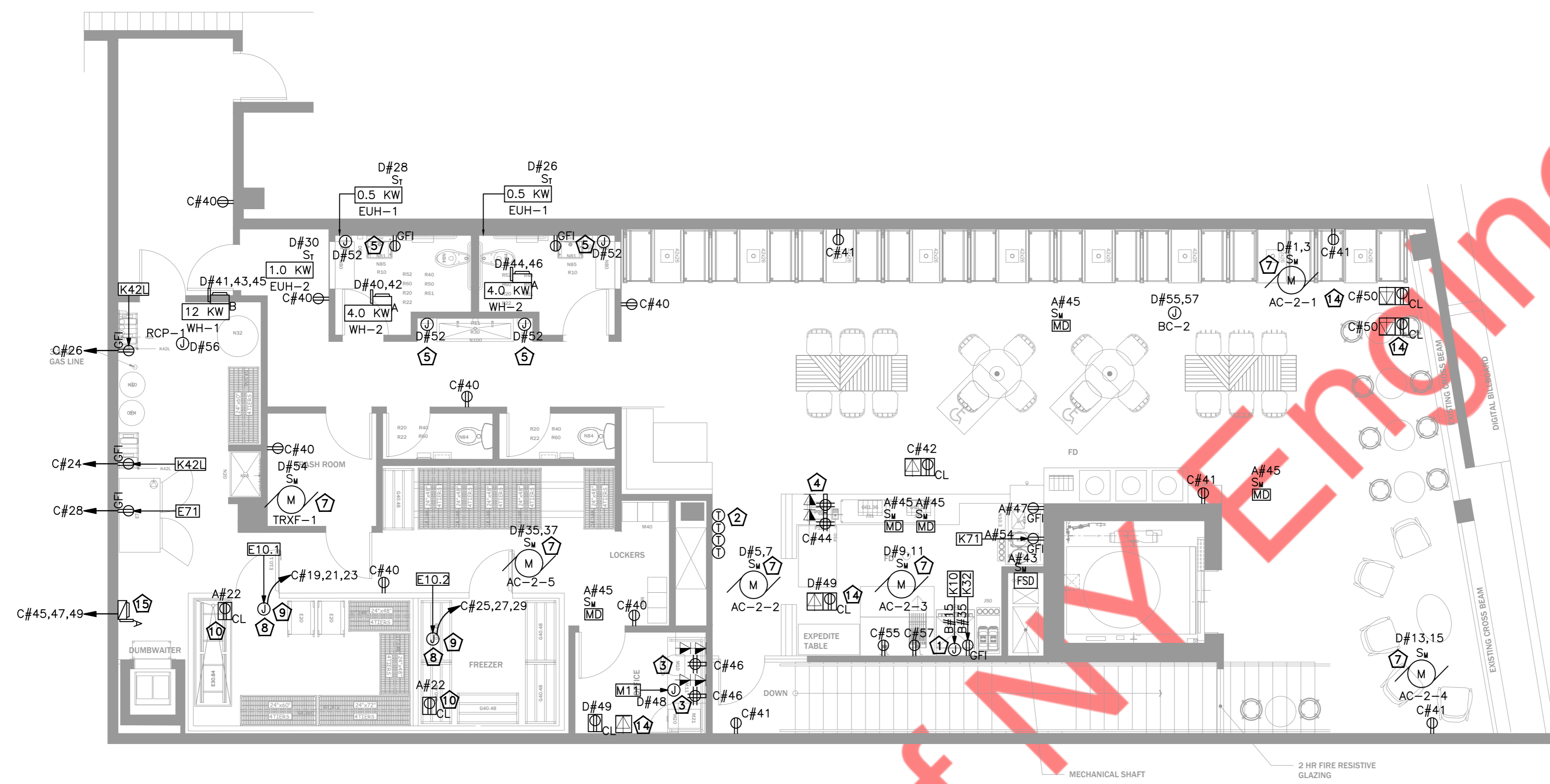
1 ELECTRICAL POWER PLAN - SECOND FLOOR E-201.00 3/16"=1'-0"
